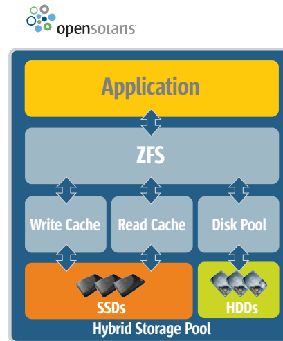
Figure 3. ZFS transparently optimizes data placement across hard disk drives and SSDs to deliver improved throughput.
